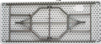
NEATLY FOLDED UNDERSIDE SHOWING LEGS, CROSSBARS & STEEL CHANNELS
